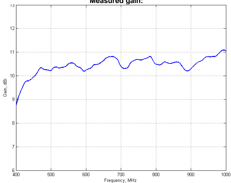
Measured gain:
