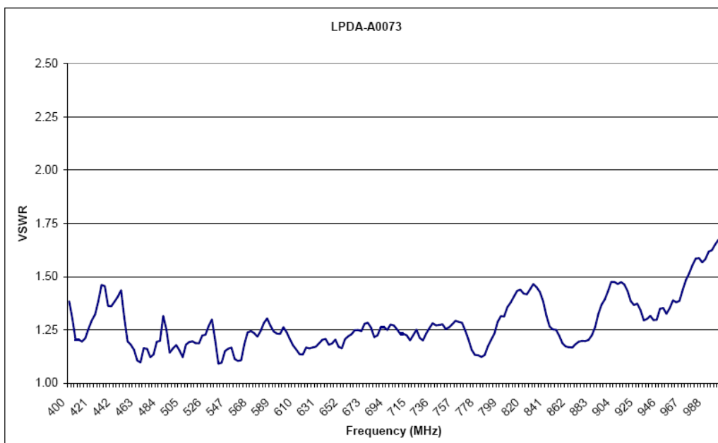
Measured VSWR:
